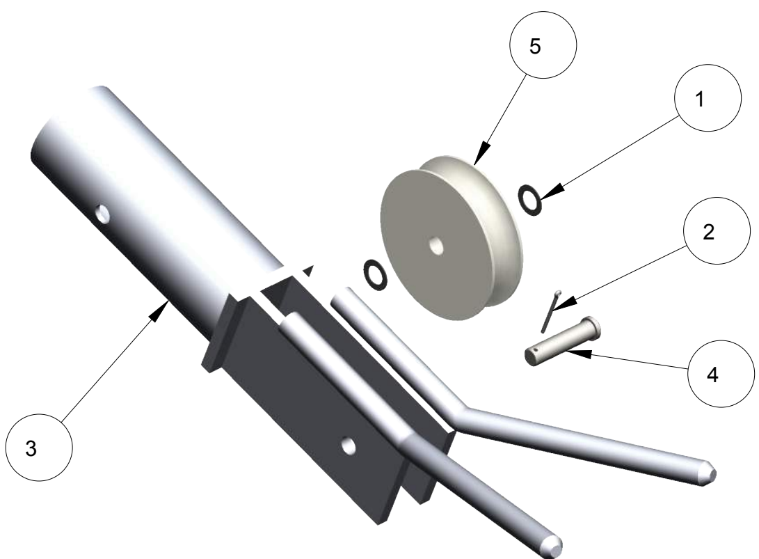
JB3010-00 (BOOM END ASSEMBLY)
