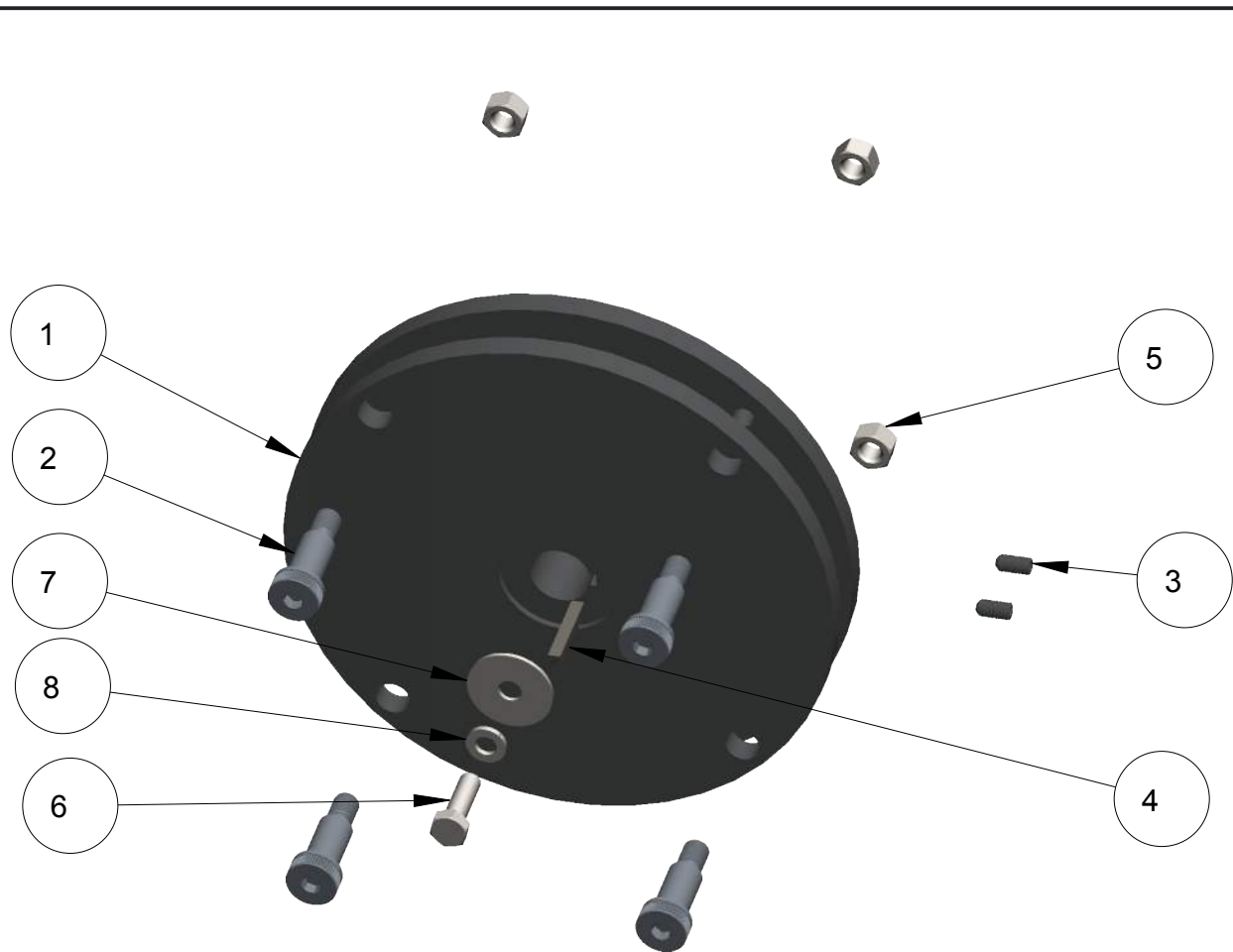
CH3019-00 (4 CHAIN STEEL FLAIL HEAD CUTTER ASSEMBLY
