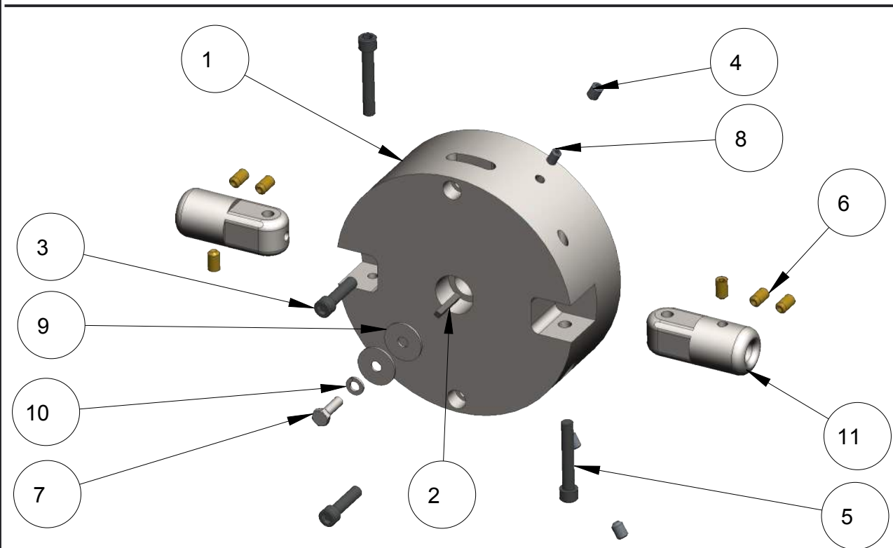
CH3020-00 (2 CHAIN & 2 WHIP ALUMINUM CUTTER HEAD ASSEMBLY
